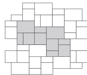
13" Soldier Course
